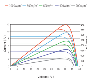
Current-Voltage &amp; Power-Voltage Curves (400W)
